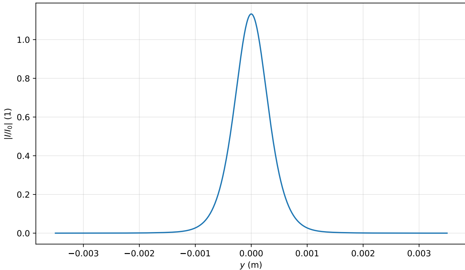
Intensity profile I(x=0, y, z=2.866)/I_0 , P_{in}=0.8P_{cr} , artificial time
